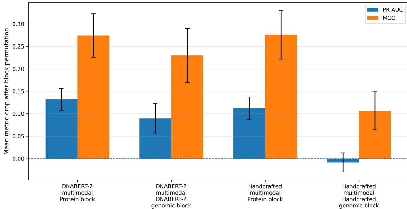
Modality Contribution by Block-Level Permutation Importance
