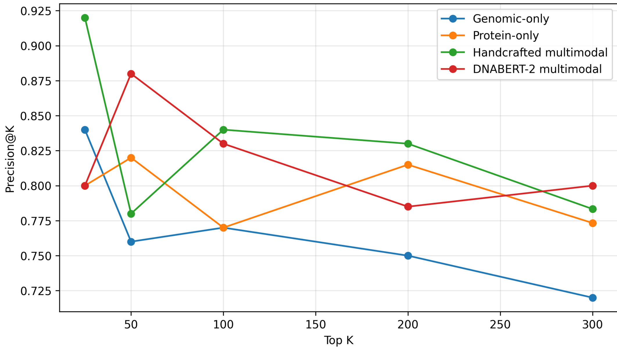
Top-K Current-Positive Recovery
