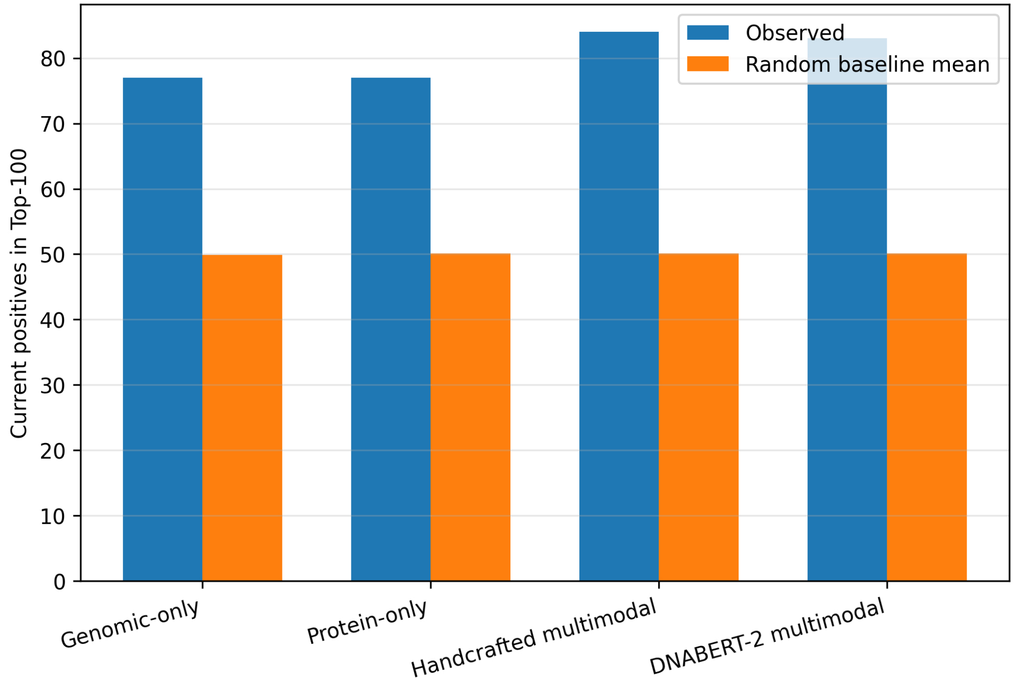
Observed vs Random Current-Positive Recovery in Top-100
