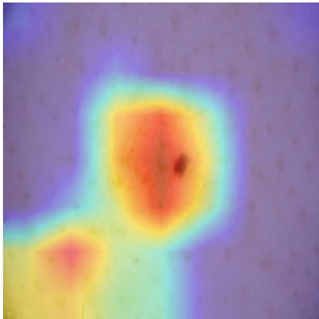
DenseNet169 P=0.211
