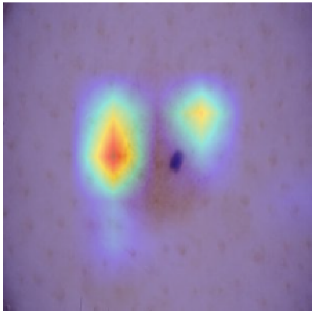
EfficientNetV2B0 P=0.242
