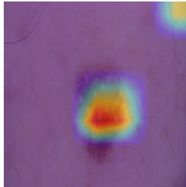
DenseNet169 P=0.102
