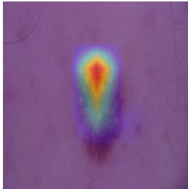
MobileNetV2 P=0.048
