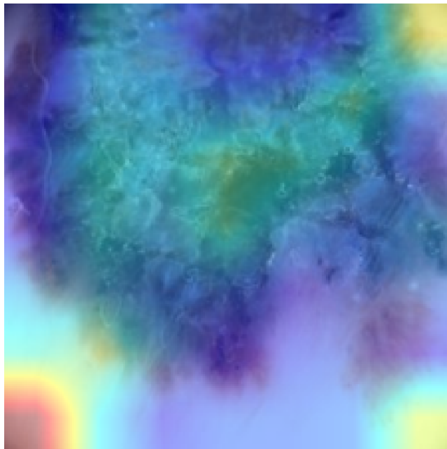
EfficientNetV2B0 P=0.996
