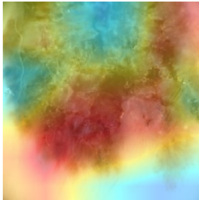
DenseNet169 P=0.996
