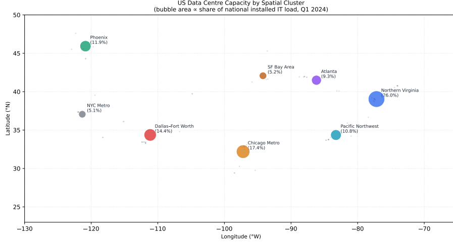
Figure 2: Weighted k -means spatial clustering ( k=8 ) of 312 US data centre facilities. Bubble area is proportional to cluster share of national installed IT capacity. Cluster centre coordinates, capacity shares, and bootstrap 95% CIs are in results/cluster_stats.csv . Code: code/02_clustering.py . Silhouette score: 0.61.
