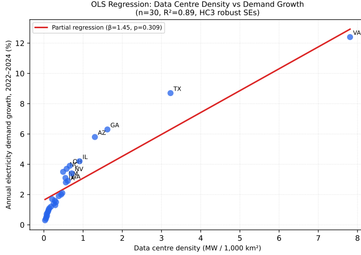
Figure 4: Partial regression plot: annual electricity demand growth vs data centre density by state (2022–2024). Red line is the OLS partial fit holding controls at their means. Selected states labelled. HC3 robust SEs; Moran’s I = 0.08 , p = 0.31 on residuals. Code: code/04_regression.py .
