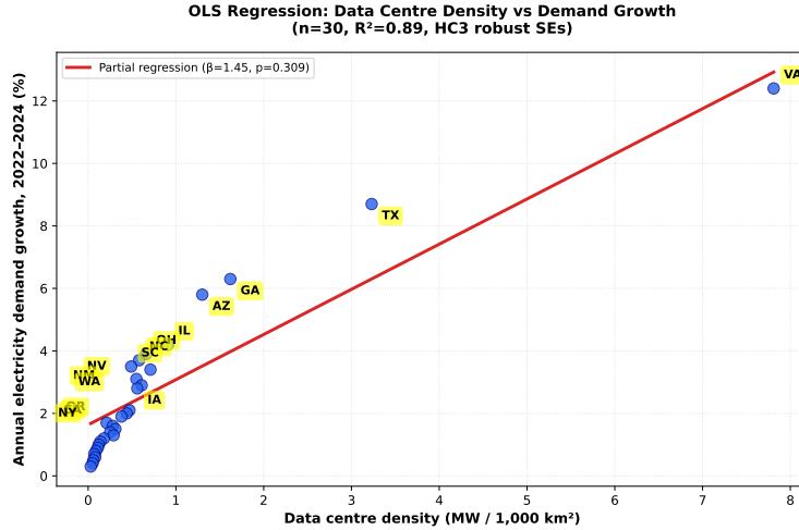
Figure 4: Partial regression plot: annual electricity demand growth vs data centre density by state (2022–2024). Red line is the OLS partial fit from the full four-predictor model, holding controls at their means. Selected states labelled. R^2 = 0.89 ; \hat{\beta}_{\text{density}} = 1.45 , p = 0.309 (HC3 robust SEs); Moran’s I = -0.17 , p > 0.05 on residuals. Code: code/04_regression.py.
