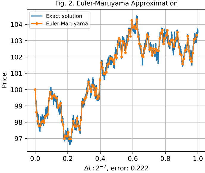
Figure 2: Euler-Maruyama Approximation
