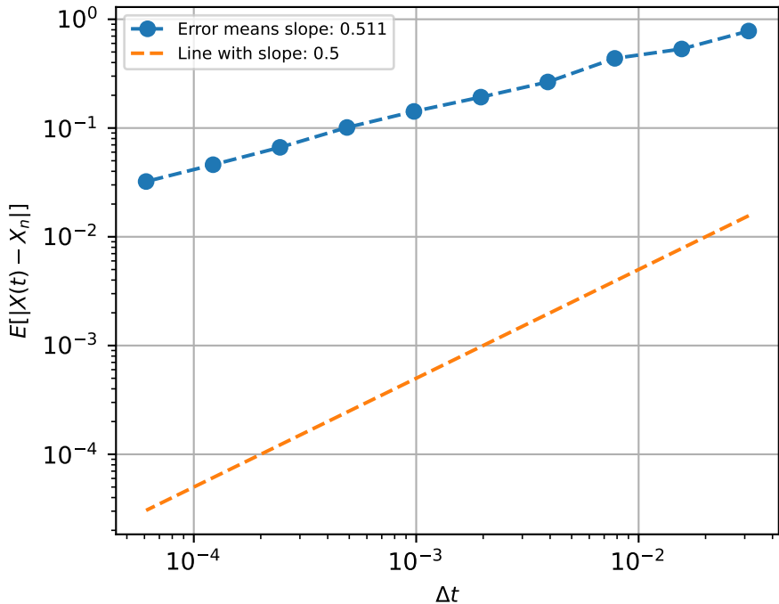
Fig. 3. Euler-Maruyama Strong Error e_{\Delta t}^{Strong} Residual: 0.052611
