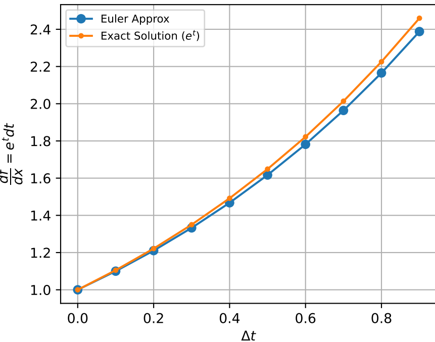
Fig.1 Euler Method for f(x) = xe^t
