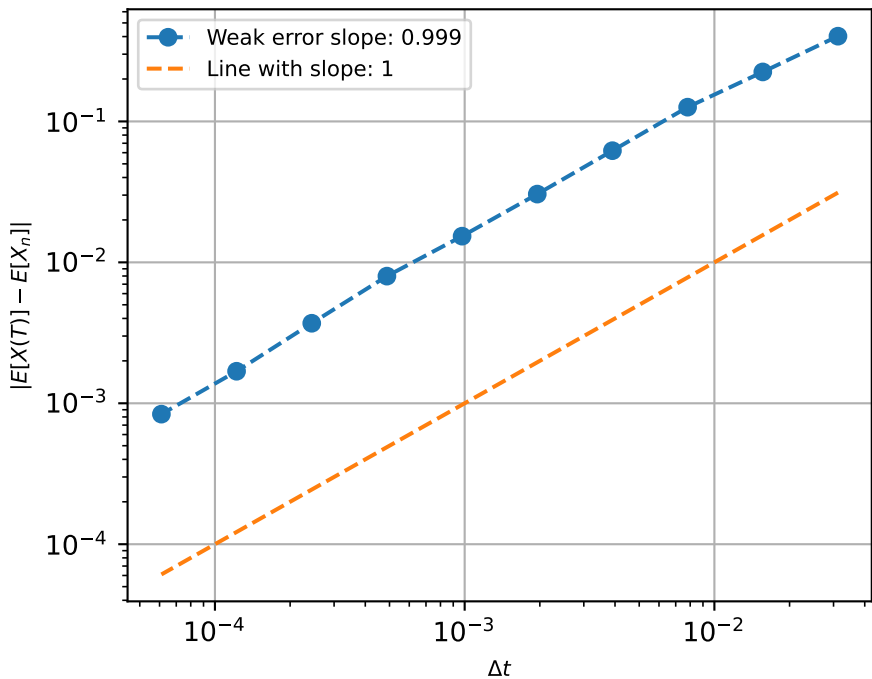
Fig. 6. Milstein Weak Error e_{\Delta t}^{Weak} Residual: 0.086131
