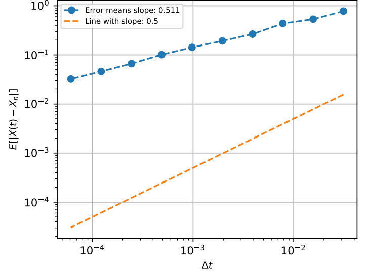
Fig. 3. Euler-Maruyama Strong Error e_{\Delta t}^{\text{Strong}} Residual: 0.052611
