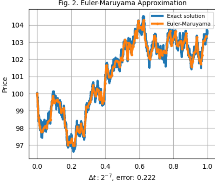
Figure 2: Euler-Maruyama Approximation
