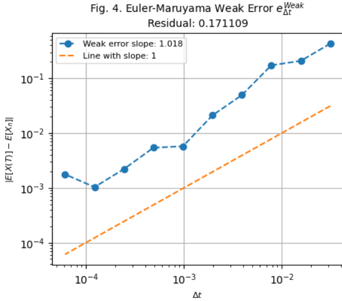
Figure 4: Euler-Maruyama Weak Error Convergence
