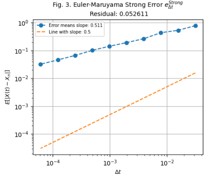
Figure 3: Euler-Maruyama Strong Error Convergence
