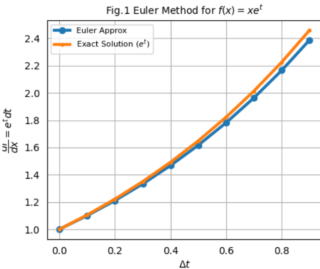
Figure 1: Euler Method
