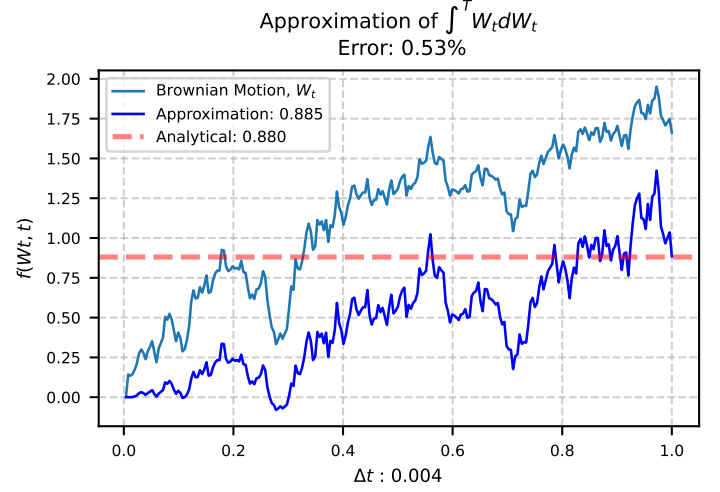
Figure 1: Approximation of Ito integral
