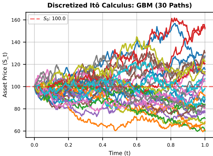
Figure 5: Ito Calculus Discrete
