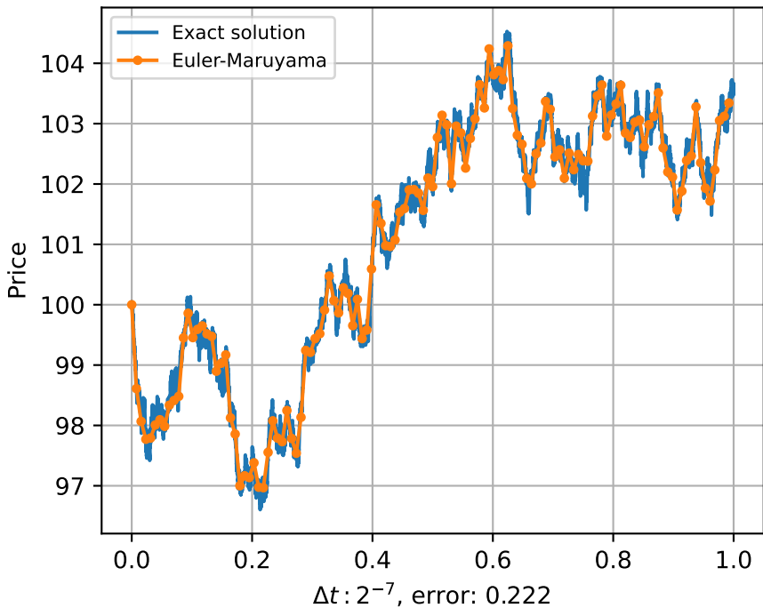
Fig. 2. Euler-Maruyama Approximation
