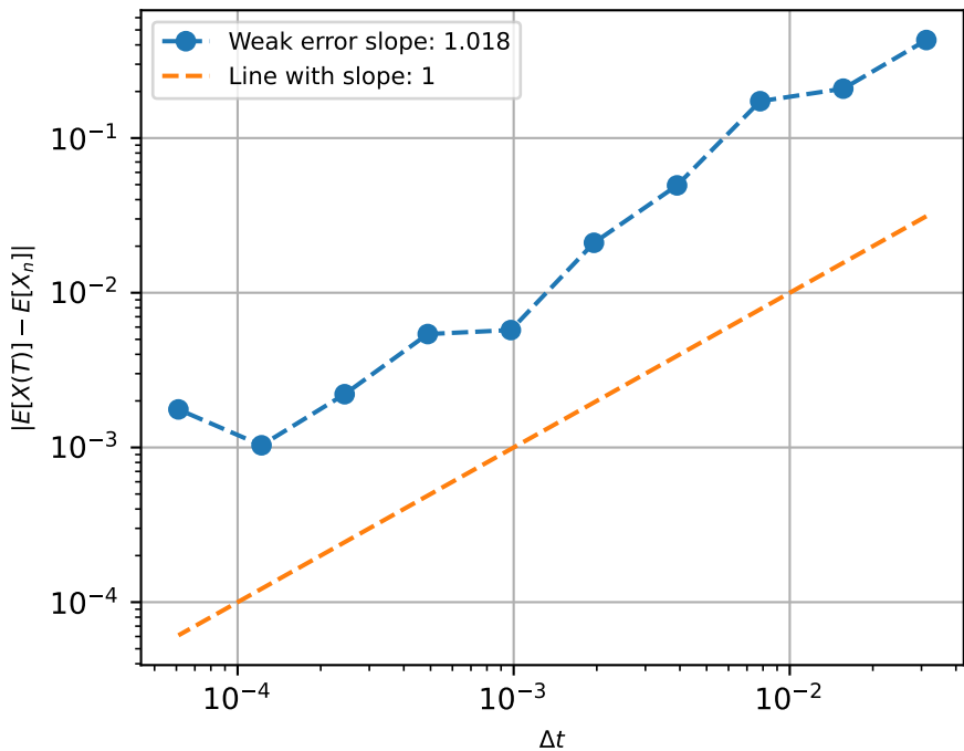
Fig. 4. Euler-Maruyama Weak Error e_{\Delta t}^{Weak} Residual: 0.171109
