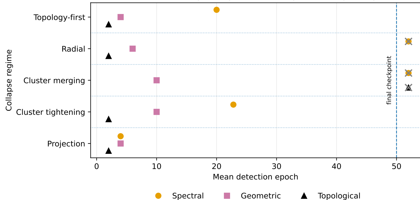
Mean detection epoch by metric family and collapse regime
