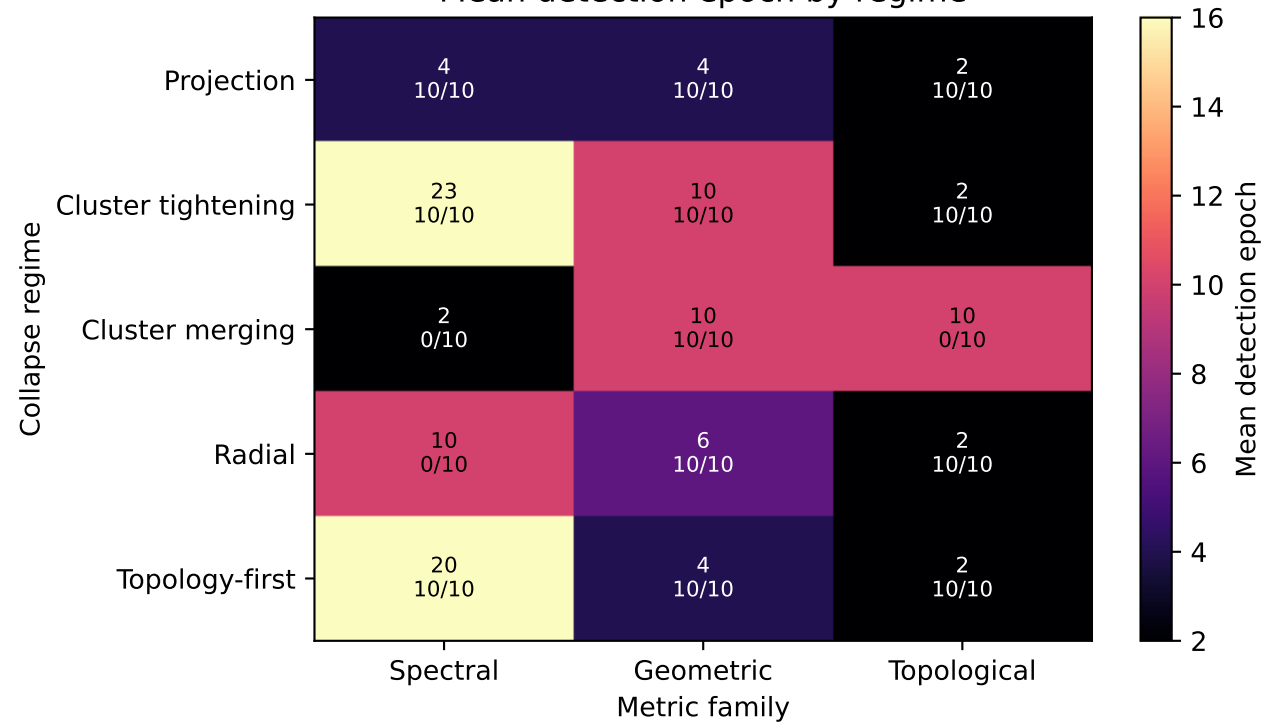
Mean detection epoch by regime
