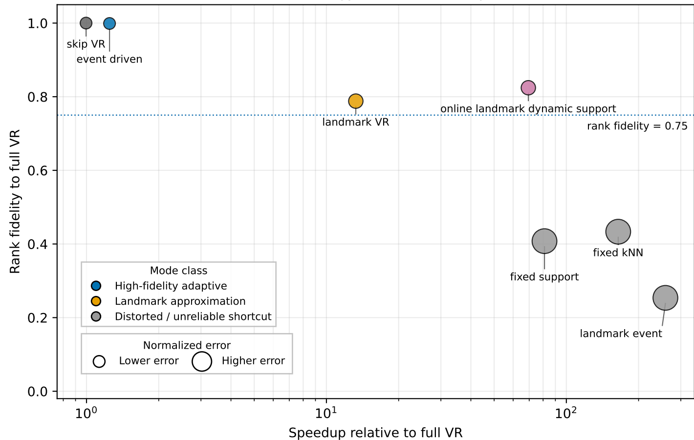
Persistent-homology runtime--fidelity tradeoff
