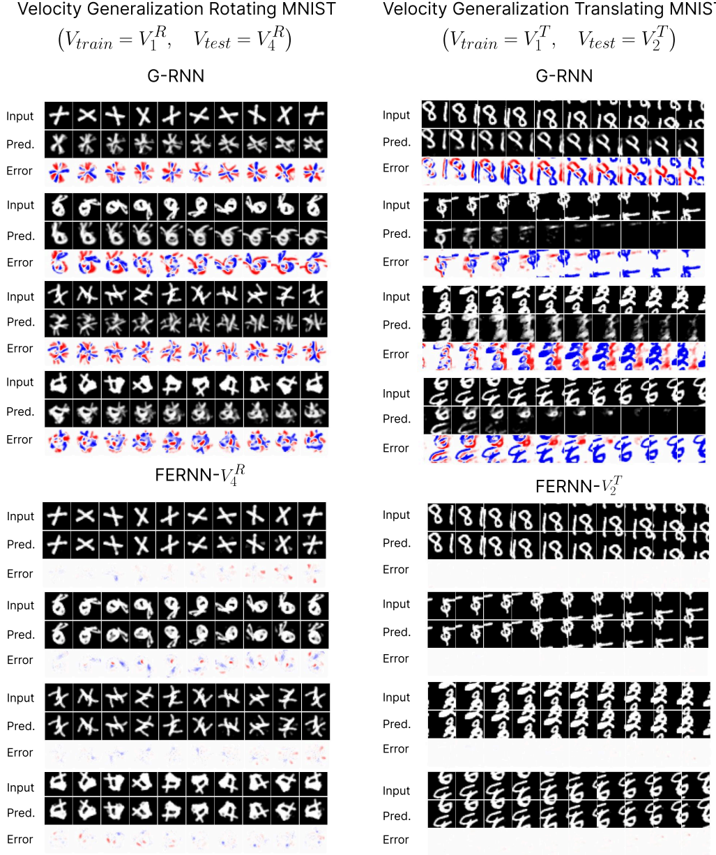
Figure 12: Samples from models trained on Rotating MNIST V_1^R (left) and Translating MNIST V_1^T (right), and tested on sequences with significantly higher velocity flows ( V_4^R and V_2^T respectively). We see that the FERNN (bottom rows) has no problem generalizing to these new velocities despite never having seen them in training, while the G-RNN (top) fails. The specific flows plotted in this example are \pm 40 \frac{\text{deg}}{\text{step}} for Rotating MNIST (left), and \nu = (\pm 2, \pm 2) for Translating MNIST.
