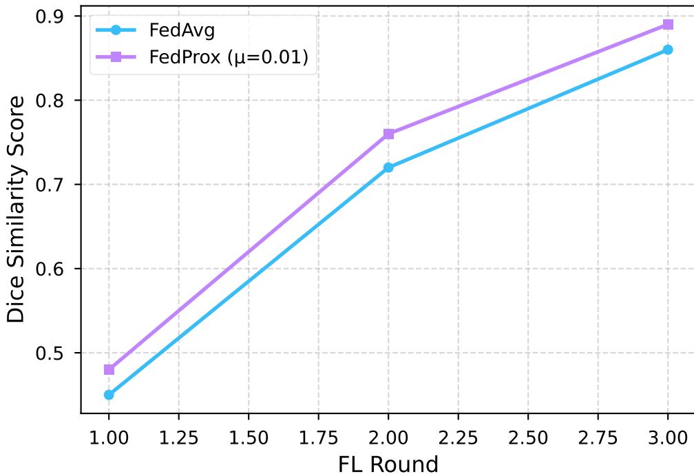
FedAvg vs FedProx Convergence Comparison
