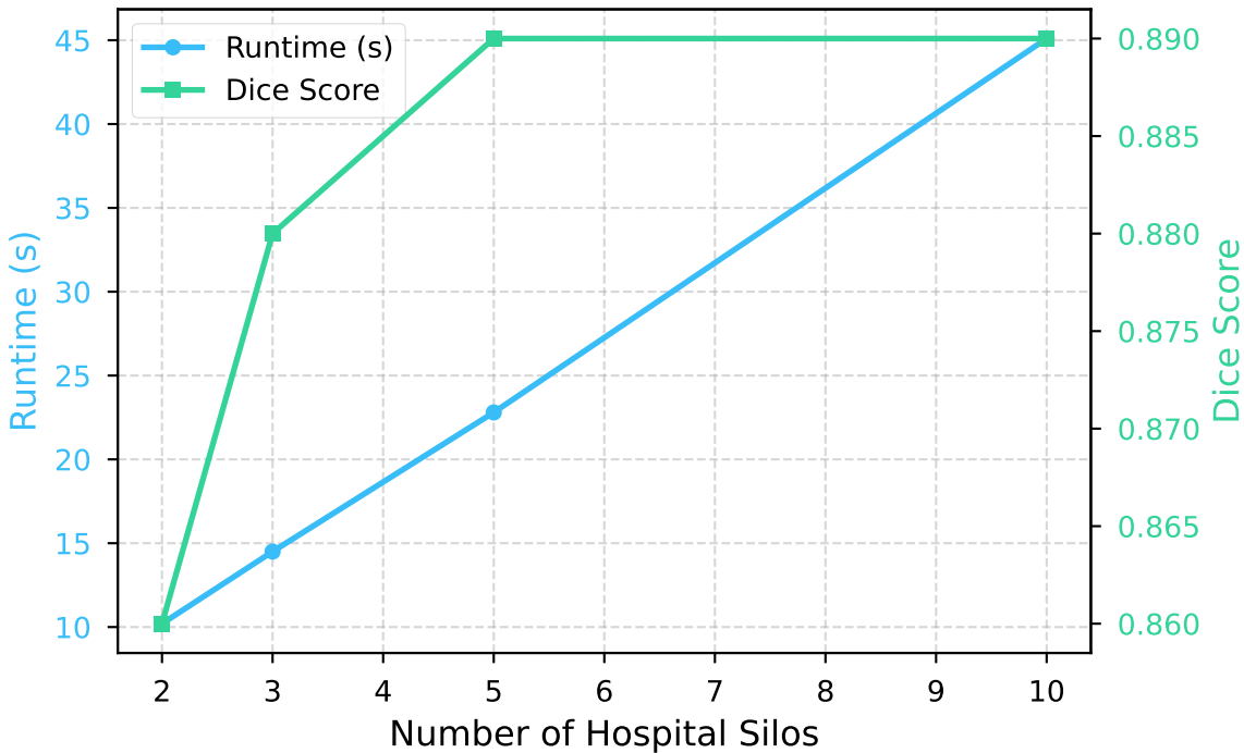
Scalability: Silos Count vs Runtime & Dice
