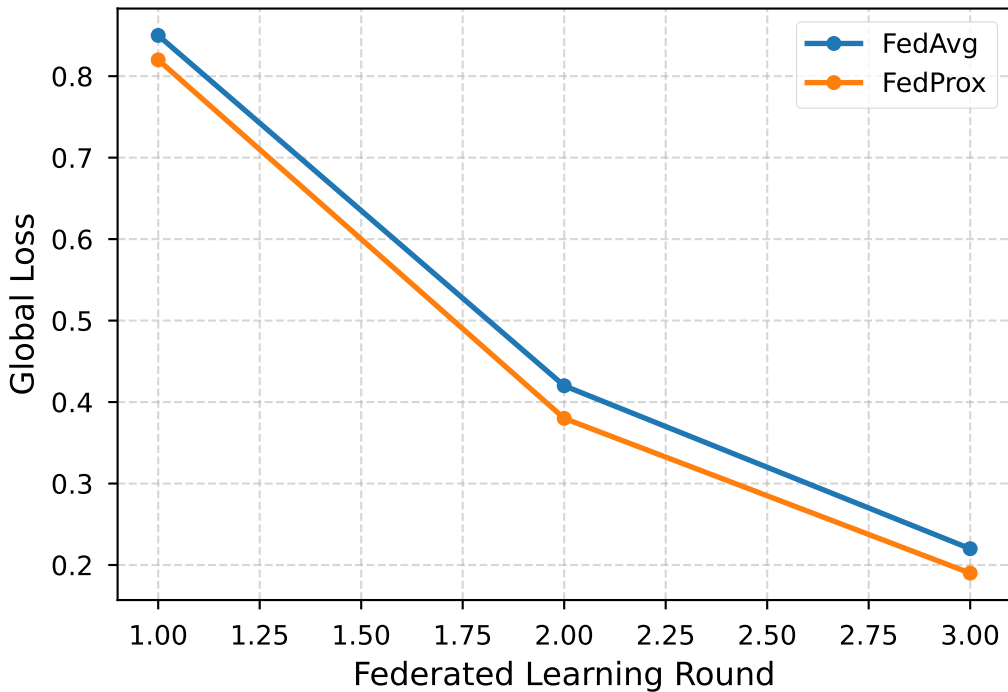
Training Loss Convergence vs FL Round
