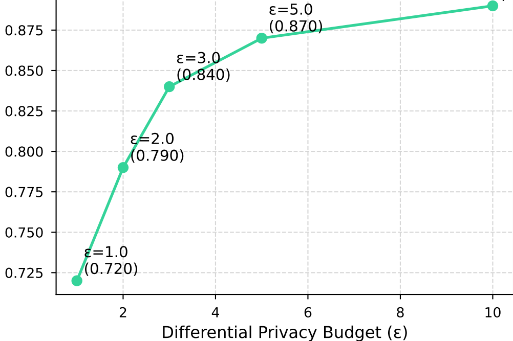
Privacy-Utility Trade-off (DP \epsilon vs Dice)
