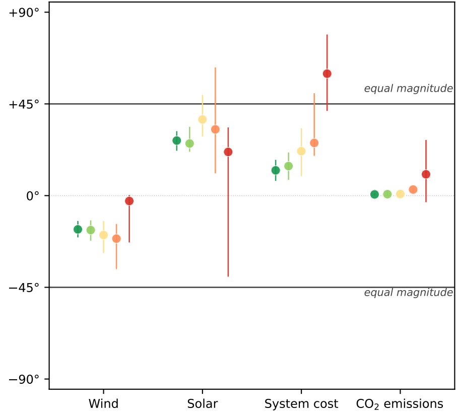
Temporal resolution (TS04→TS72)
