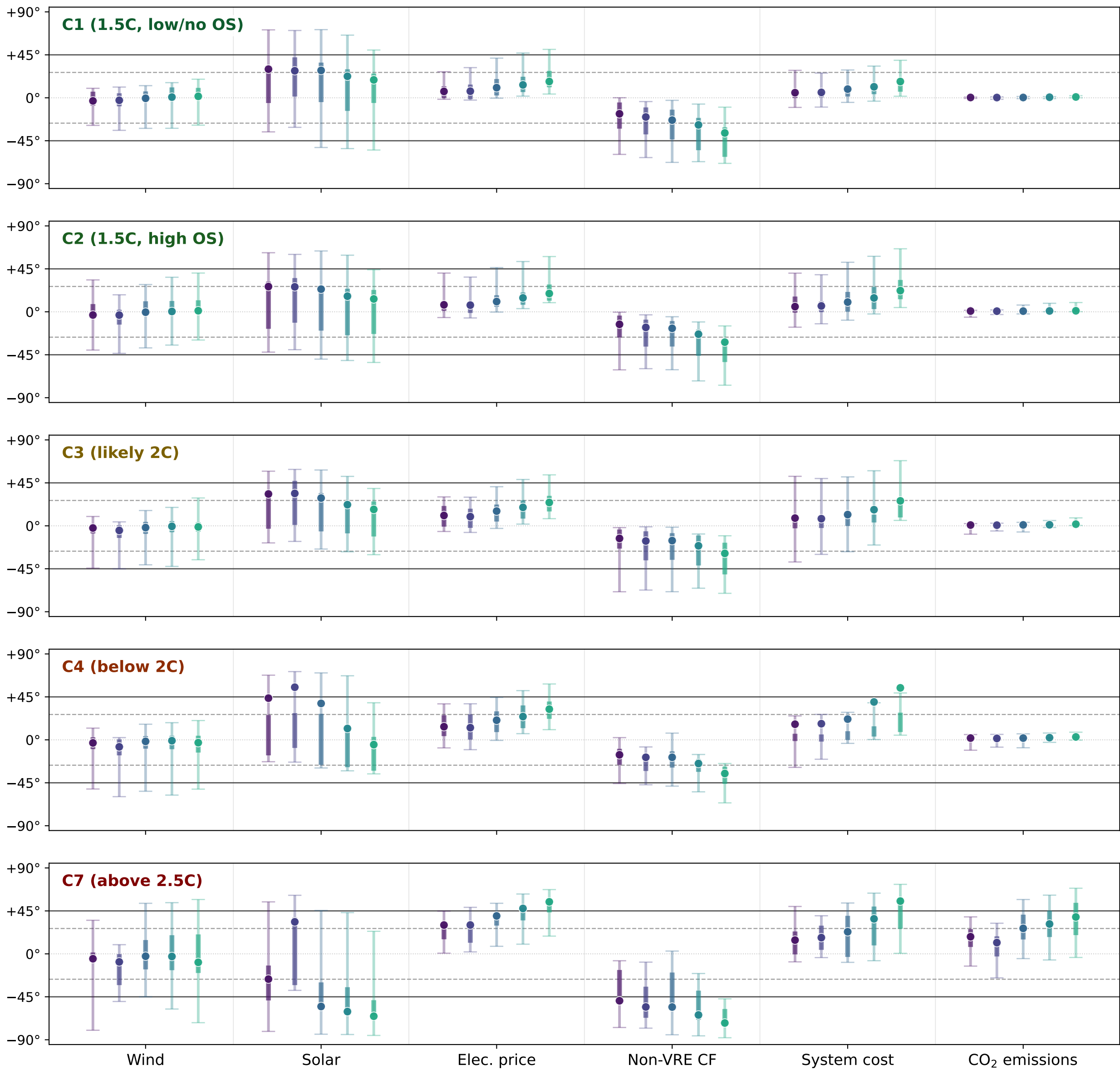
Temporal-resolution saturation: signed structural-parametric angle ( \theta ), stratified by climate category
