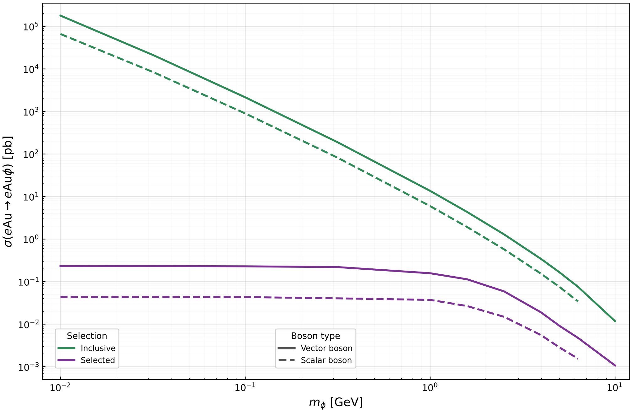
Vector and scalar signal production, g_{V(S)}^e = 10^{-4}
