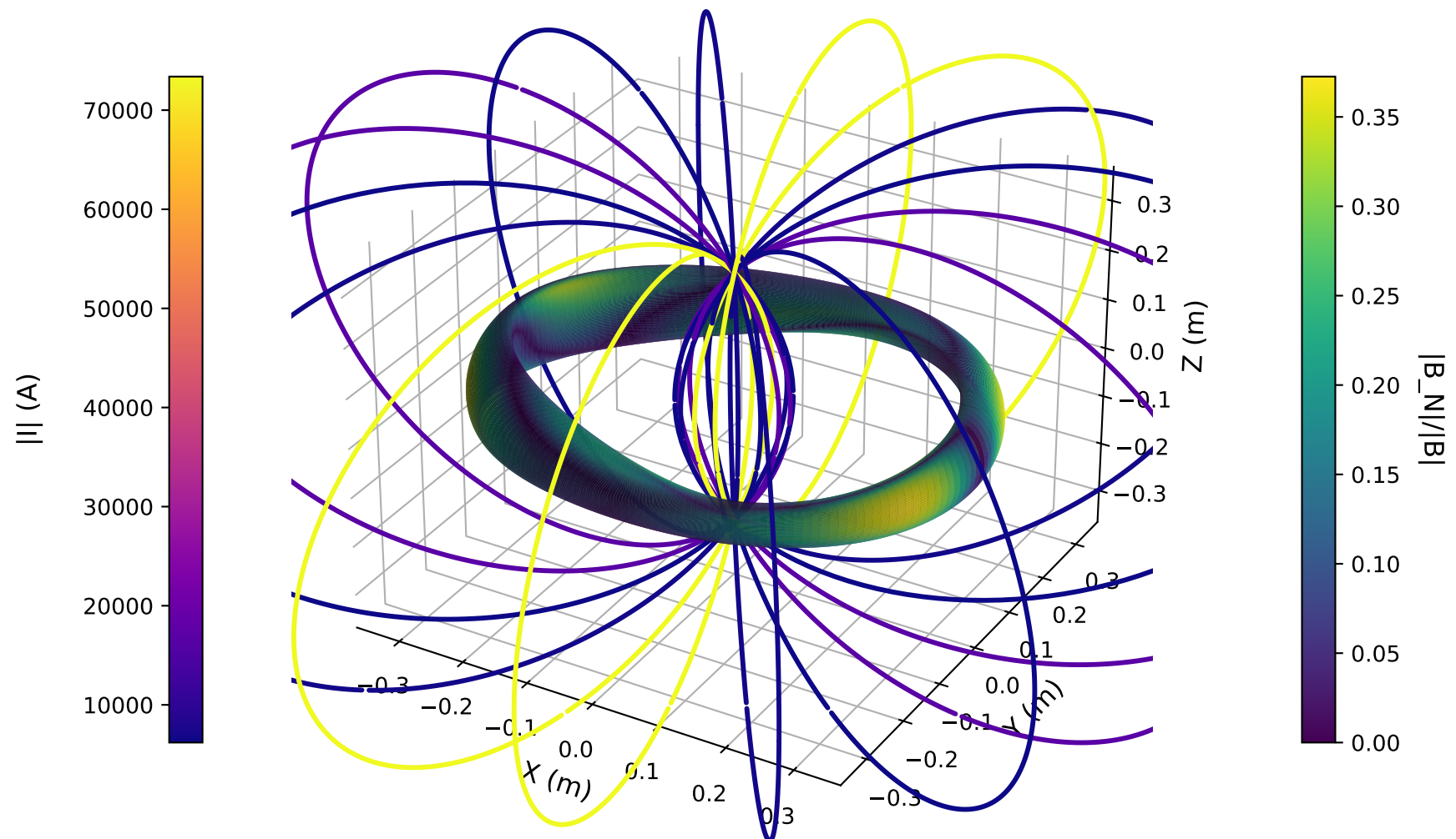
B_N/|B| Error on Plasma Surface with Optimized Coils
