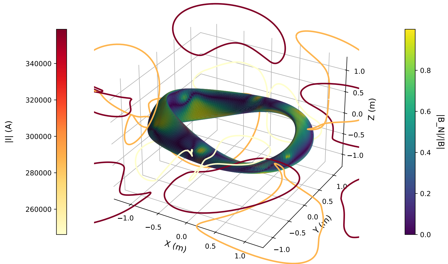
B_N/|B| Error on Plasma Surface with Initial Coils
