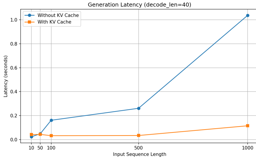
Figure 3: Latency comparison with and without KV Cache across various sequence lengths.
