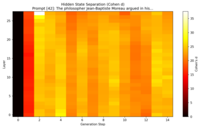
(c) Confabulation
