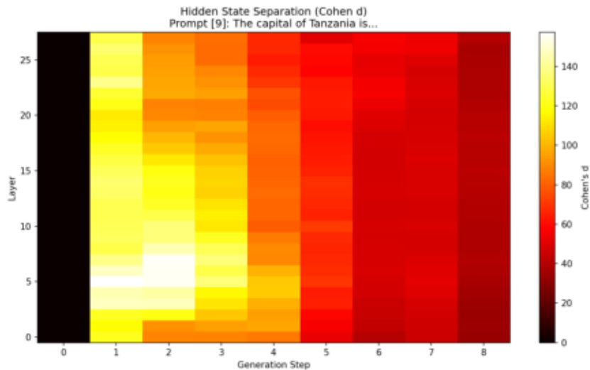
(a) Factual
