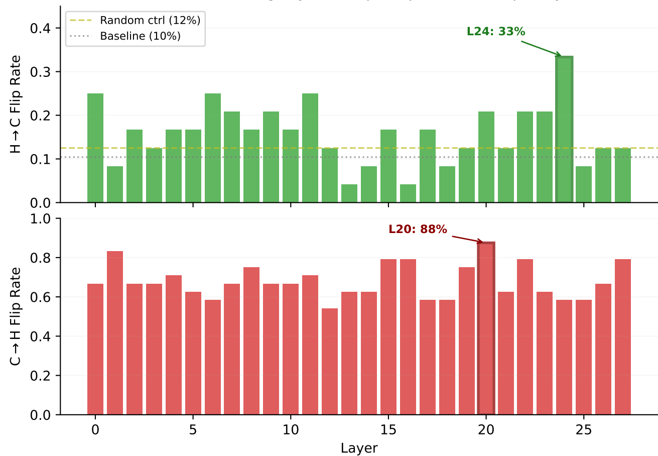
Activation Patching Layer Sweep (step = 1, n = 24 per layer)
