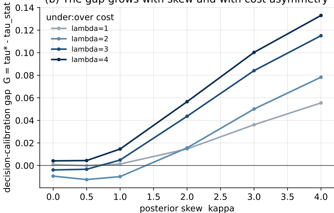
(b) The gap grows with skew and with cost asymmetry
