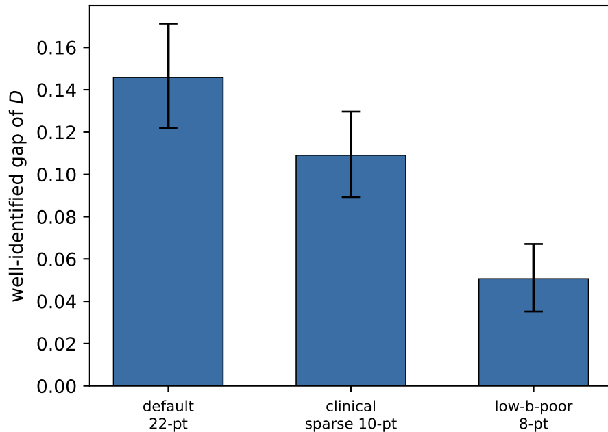
Robust across acquisition schemes (all survive; weakest when low-b is sparse)
