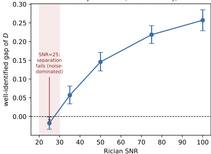
Separation intensifies with SNR; fails only at SNR=25 (honest boundary)
