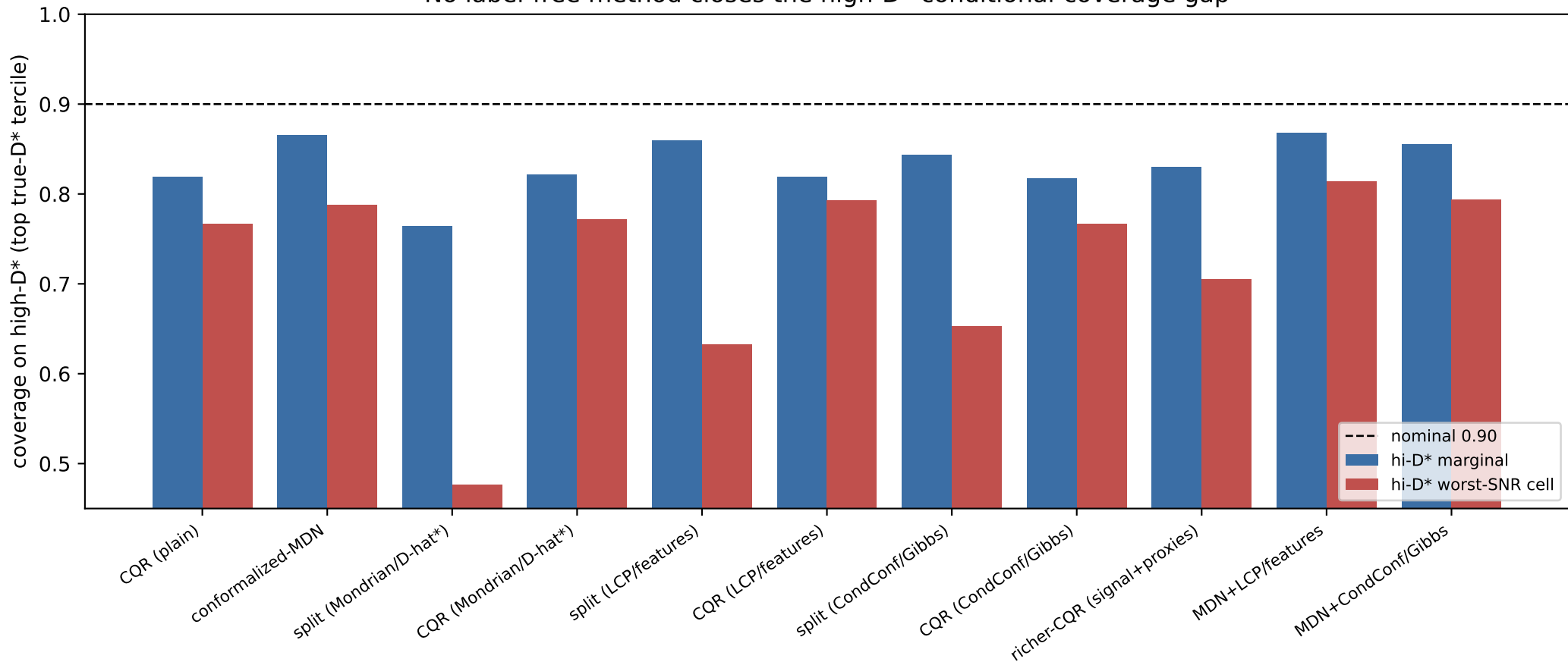
No label-free method closes the high- D^* conditional-coverage gap
