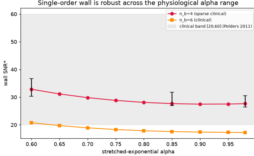
Figure 2: The single-order wall SNR* versus the stretched-exponential order \alpha at sparse clinical acquisition (with bootstrap CIs at representative \alpha ), inside the cited clinical-SNR band (shaded) across the whole physiological range.
