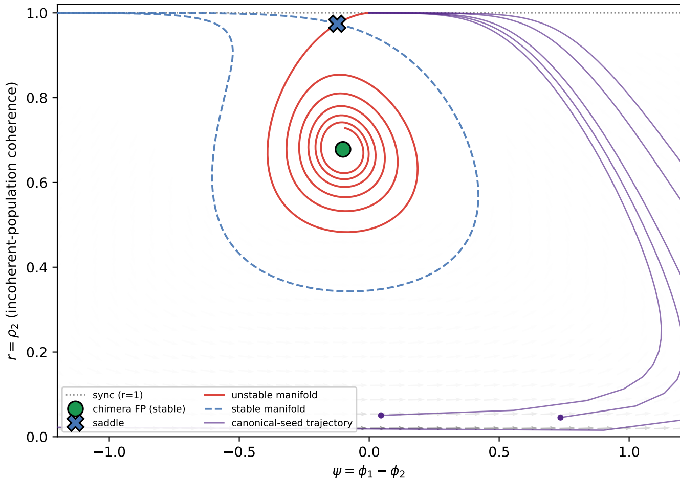
2-D phase portrait A=0.2, \beta=0.05 (stable stationary chimera)
