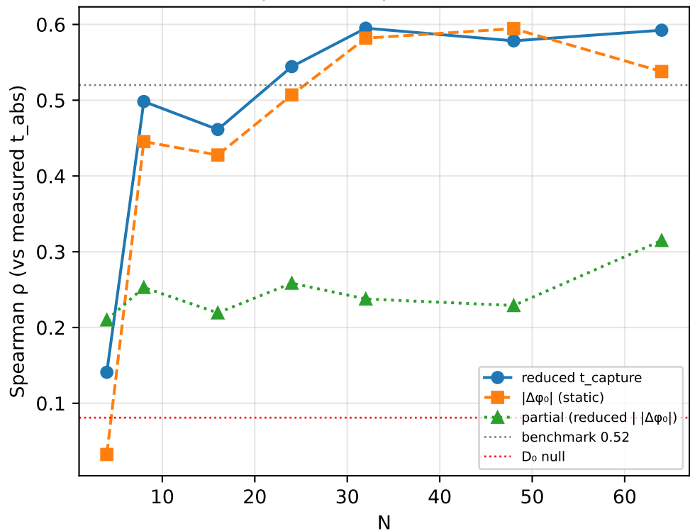
predictive power vs N
