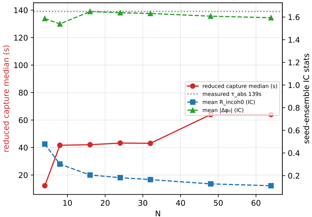
where N enters: seed-ensemble ICs vs dynamics
