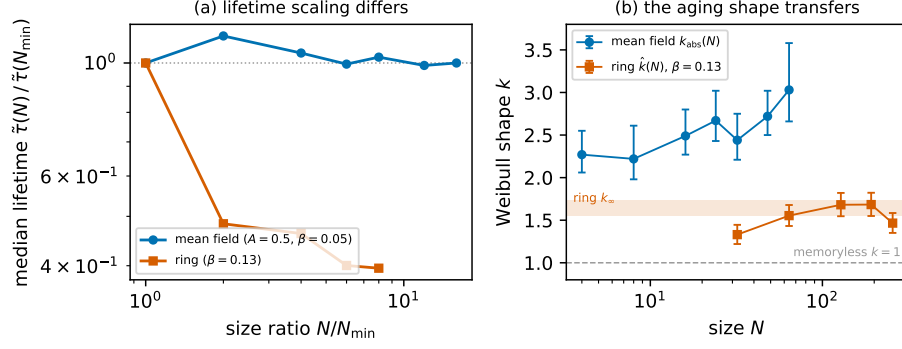
Fig. 12 Cross-system comparison: aging transfers, scaling does not. (a) Median lifetime versus size, each system normalized to its smallest campaign size: the mean-field absorption plateau is flat over a 16\times range of N ( \bar{\tau}(64)/\bar{\tau}(4) = 1.00 ), while the ring’s near-boundary median falls 2.5\times over an 8\times range ( 872 \rightarrow 345 time units at \beta = 0.130 ). (b) Censored-Weibull shape versus size for the same campaigns: mean-field k_{\text{abs}} = 2.27\text{--}3.03 and ring \hat{k} = 1.33\text{--}1.68 , every interval above the memoryless k = 1 (dashed); the band is the ring’s bootstrapped thermodynamic limit k_\infty = 1.65 [ 1.56, 1.74 ] at \beta = 0.130 (Appendix D).
