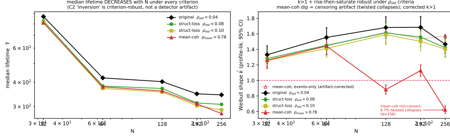
Fig. D5 Criterion-independence at \beta = 0.130 . Left: median lifetime decreases with N under every death criterion (the near-boundary inversion is not a detector artifact). Right: the Weibull shape \hat{k}(N) stays above one under the spatial-homogeneity ( \rho_{\text{std}} ) criteria; the mean-coherence rule’s apparent dip below one at large N is a censoring artifact (twisted-state collapses mislabeled as censored), and the artifact-corrected curve returns above one.
