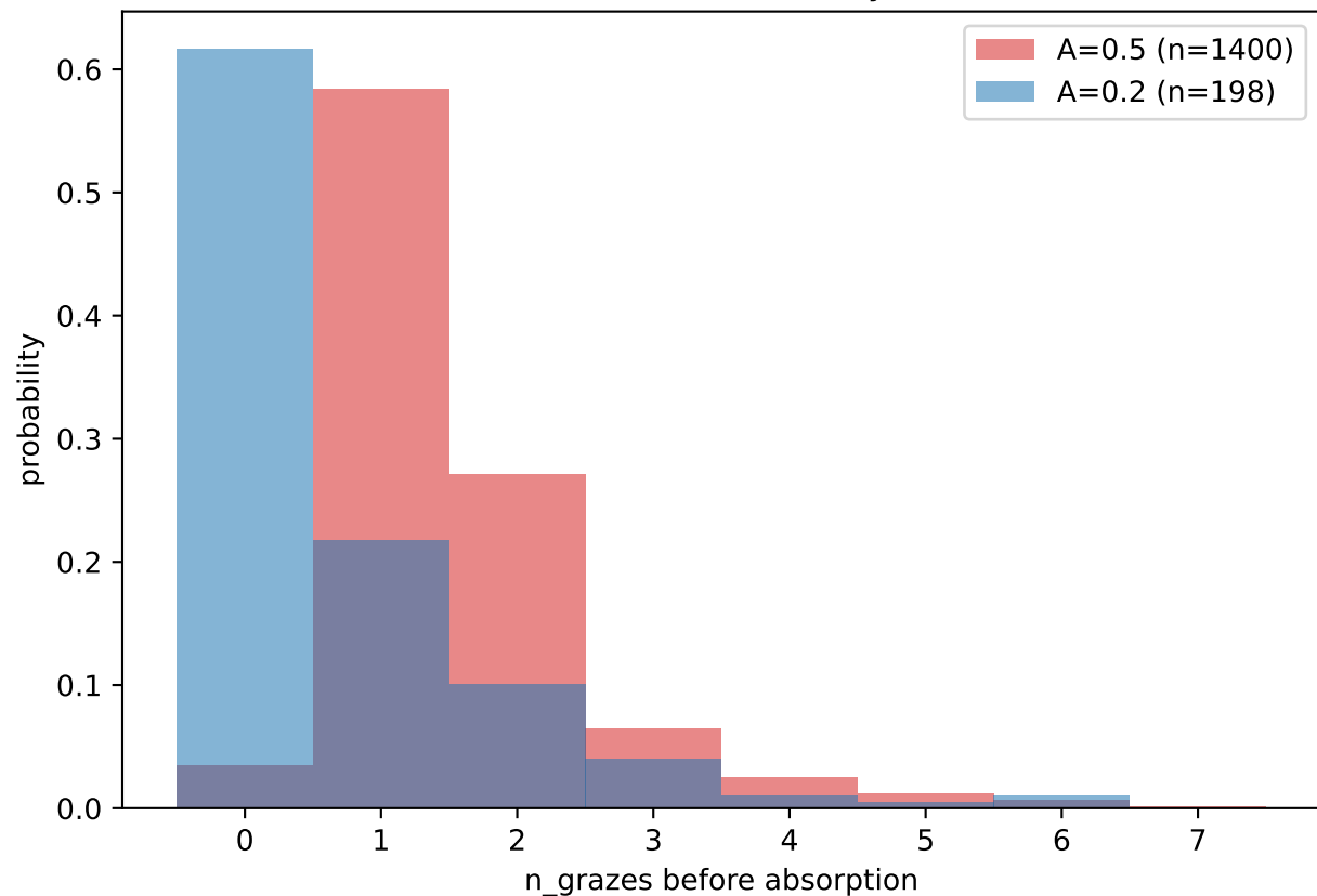
Grazes before a true absorption (absorbed runs only)
