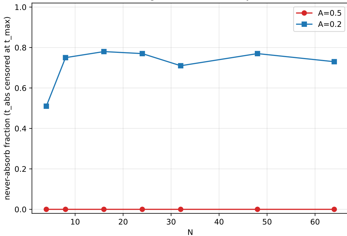
Graze-survival fraction vs N (fraction that grazes but never truly absorbs)
