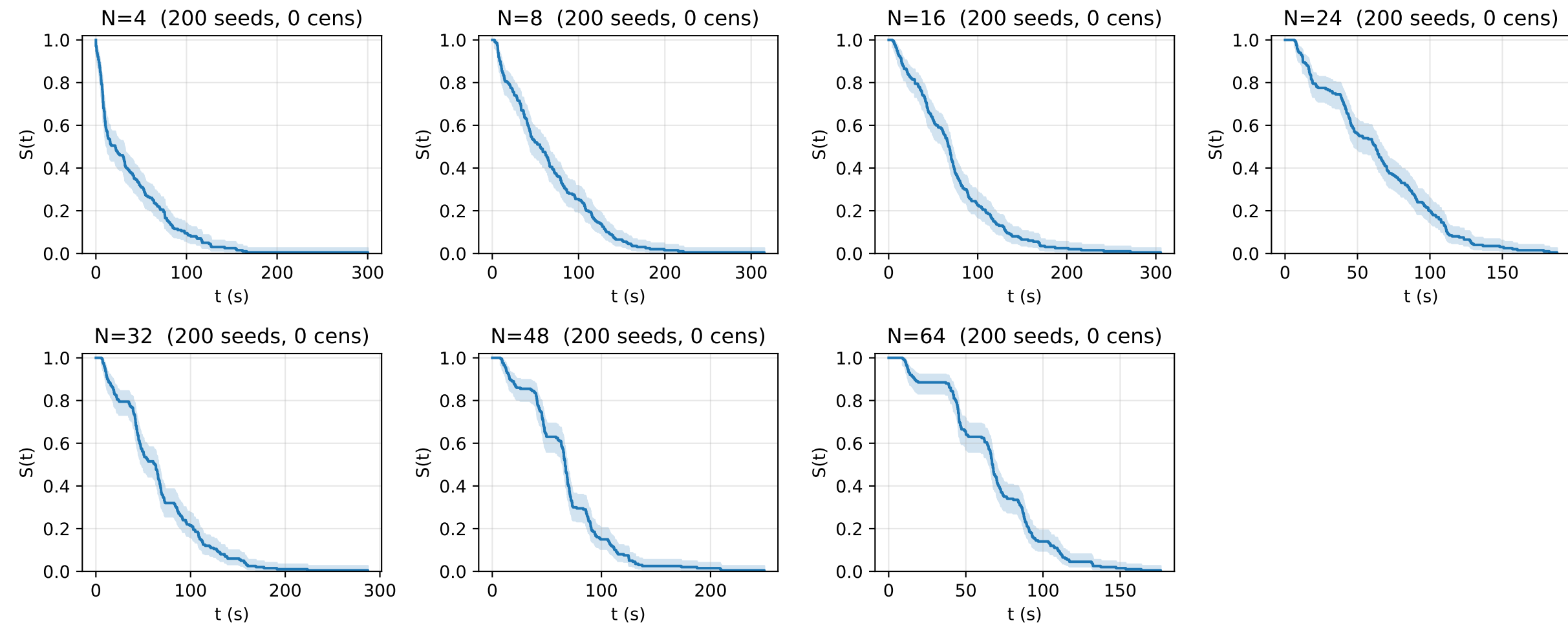
Kaplan-Meier survival — A=0.5 (primary), \beta=0.05
