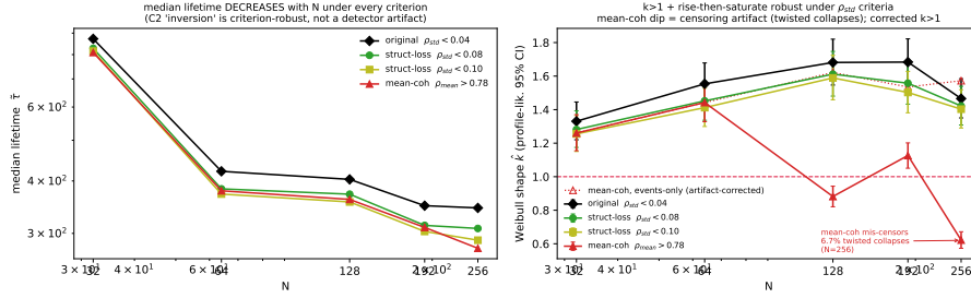
Fig. D6 Criterion-independence at \beta = 0.130 . Left: median lifetime decreases with N under every death criterion (the near-boundary inversion is not a detector artifact). Right: the Weibull shape \hat{k}(N) stays above one under the spatial-homogeneity ( \rho_{std} ) criteria; the mean-coherence rule’s apparent dip below one at large N is a censoring artifact (twisted-state collapses mislabeled as censored), and the artifact-corrected curve returns above one.
