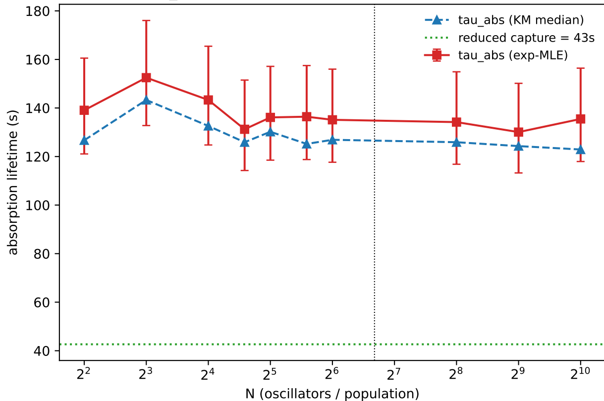
tau_abs(N) — plateau extended 16x to N=1024
