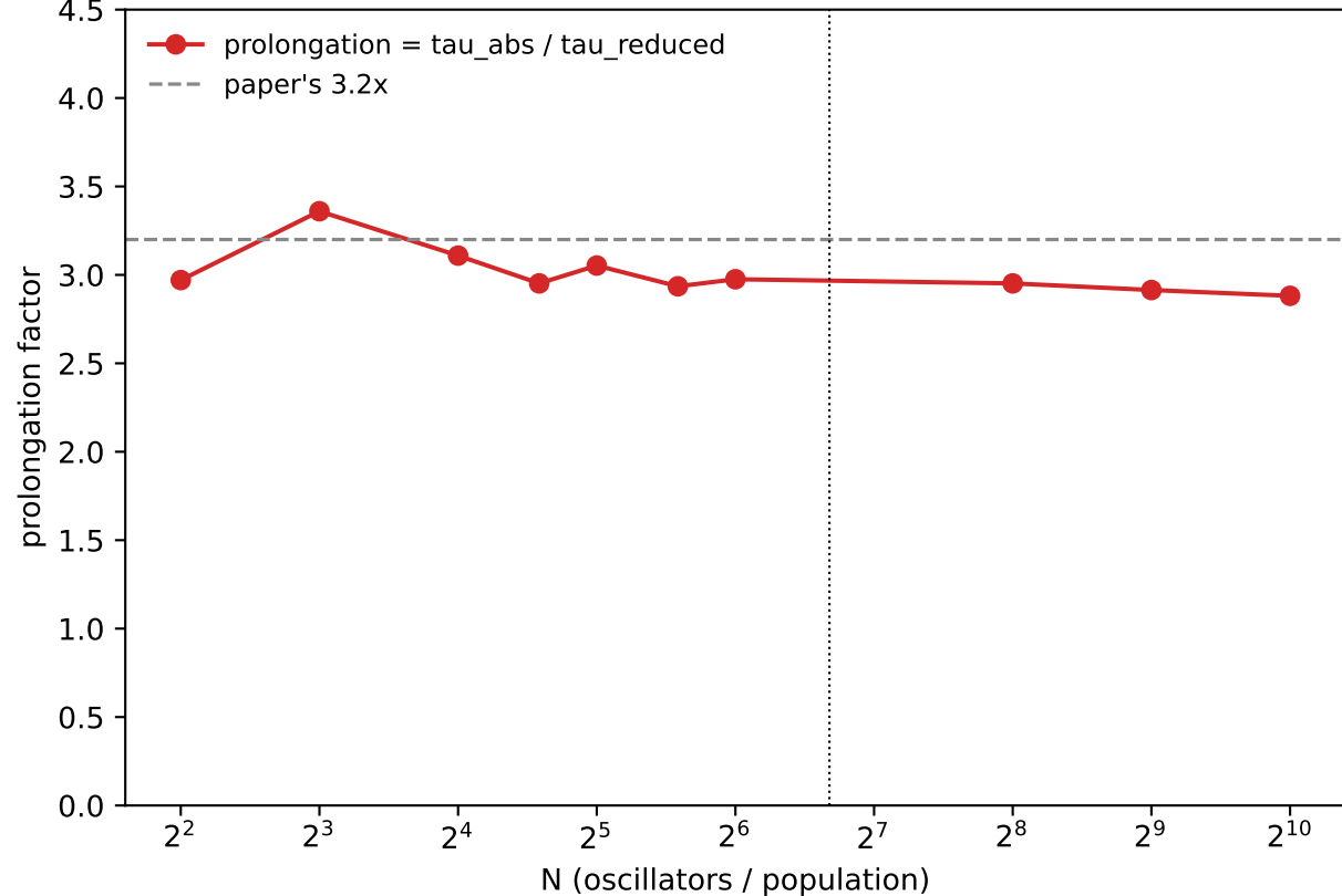
Reduced-to-finite-N prolongation vs N
