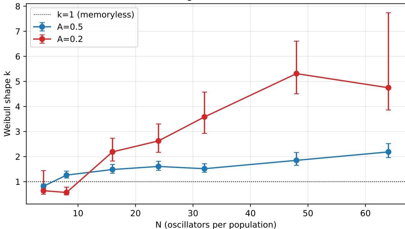
CP5 — aging vs N: Weibull shape k(N) ( k > 1 \Rightarrow increasing hazard / survival shoulder)
