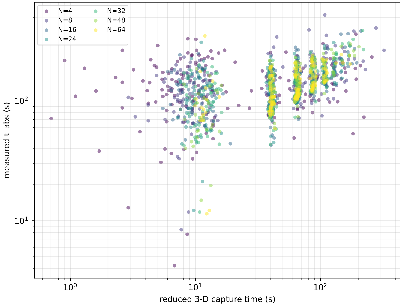
Reduced-predicted vs measured lifetime ( A=0.5 , \beta=0.05 ) pooled Spearman \rho=0.445 ( |\Delta\phi_0| benchmark \rho\approx0.52 )
