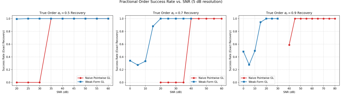
Figure 5: Order recovery success rate (exact recovery rate over 500 trials) versus SNR (dB) for Naive Pointwise GL and Weak-Form GL across true fractional orders \alpha_t \in \{0.5, 0.7, 0.9\} .
