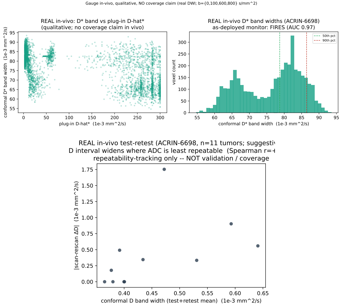
Figure 9: Real in-vivo data (ACRIN-6698 / I-SPY2 Breast DWI; qualitative, no coverage claim). (Top left) the re-fit conformal D^* band vs the plug-in \hat{D}^* ; (top right) the D^* band-width distribution and the as-deployed monitor verdict (fires, AUC 0.97, via the b -independent Mahalanobis family). (Bottom) test–retest: the conformal D -width vs the measured scan–rescan ADC variability across n=11 tumors (Spearman r = +0.69 ; suggestive, repeatability-tracking only—not validation or coverage).
