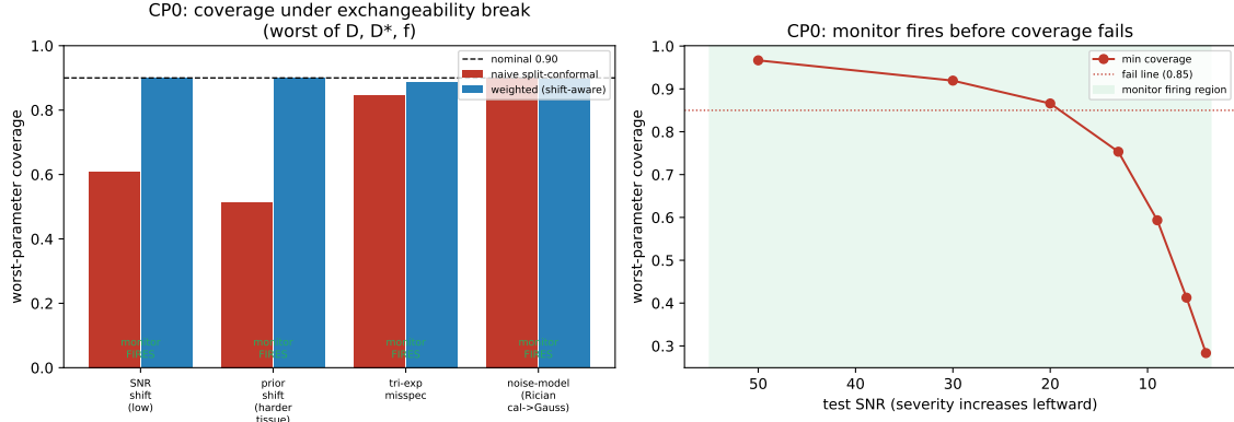
Figure 6: (Left) worst-parameter coverage under each exchangeability break, naive vs. weighted, with monitor status. (Right) SNR-severity sweep: the monitor fires before coverage crosses the failure line.
