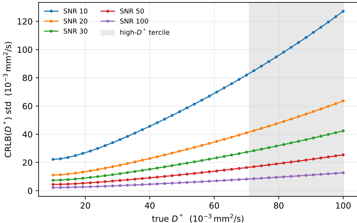
IVIM pseudo-diffusion identifiability wall (CRLB, S0 free)
