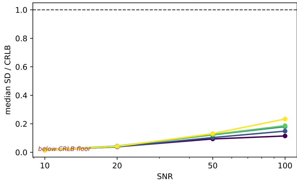
D* achieved scatter (emp_sd / CRLB)
