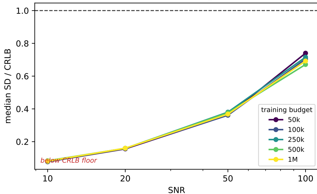
D* claimed precision (post_sd / CRLB)
