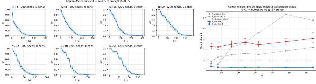
FIG. 3. Absorption survival and aging. Kaplan–Meier survival curves by N (left, A = 0.5 ) develop a shoulder with increasing N ; censored-Weibull shape k_{\text{abs}}(N) (right) rises from 2.3 to 3.0 with all confidence intervals above the memoryless value k = 1 .
