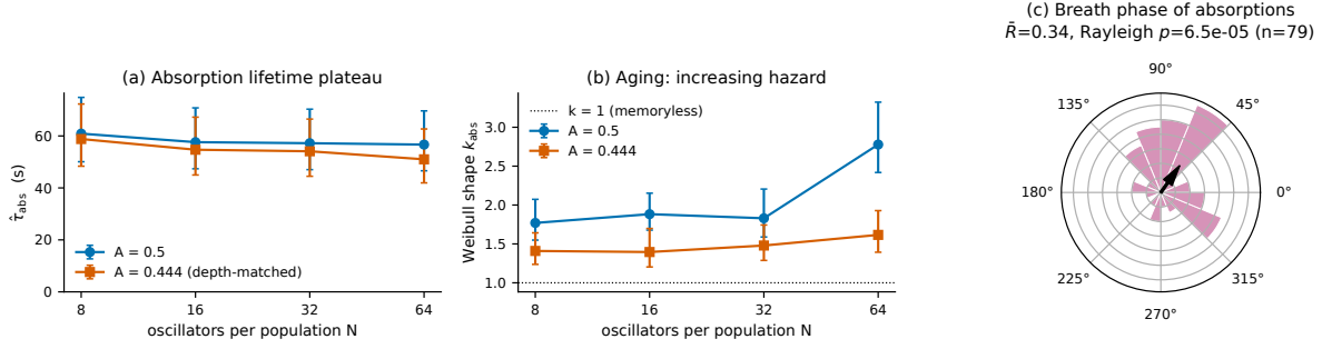
FIG. 10. Robustness at \beta = 0.10 . (a) Absorption lifetime \hat{\tau}_{\text{abs}}(N) is flat in N at both the post-homoclinic corner A = 0.5 and the depth-matched A = 0.444 . (b) Censored-Weibull shape k_{\text{abs}}(N) stays above the memoryless value k = 1 (aging persists). (c) True-absorption breath phases remain clustered (pooled \bar{R} = 0.34 , Rayleigh p = 6.5 \times 10^{-5} , n = 79 ).
